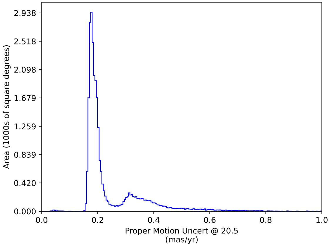
roll_3_v3.4_10yrs : Proper Motion Uncert @ 20.5
