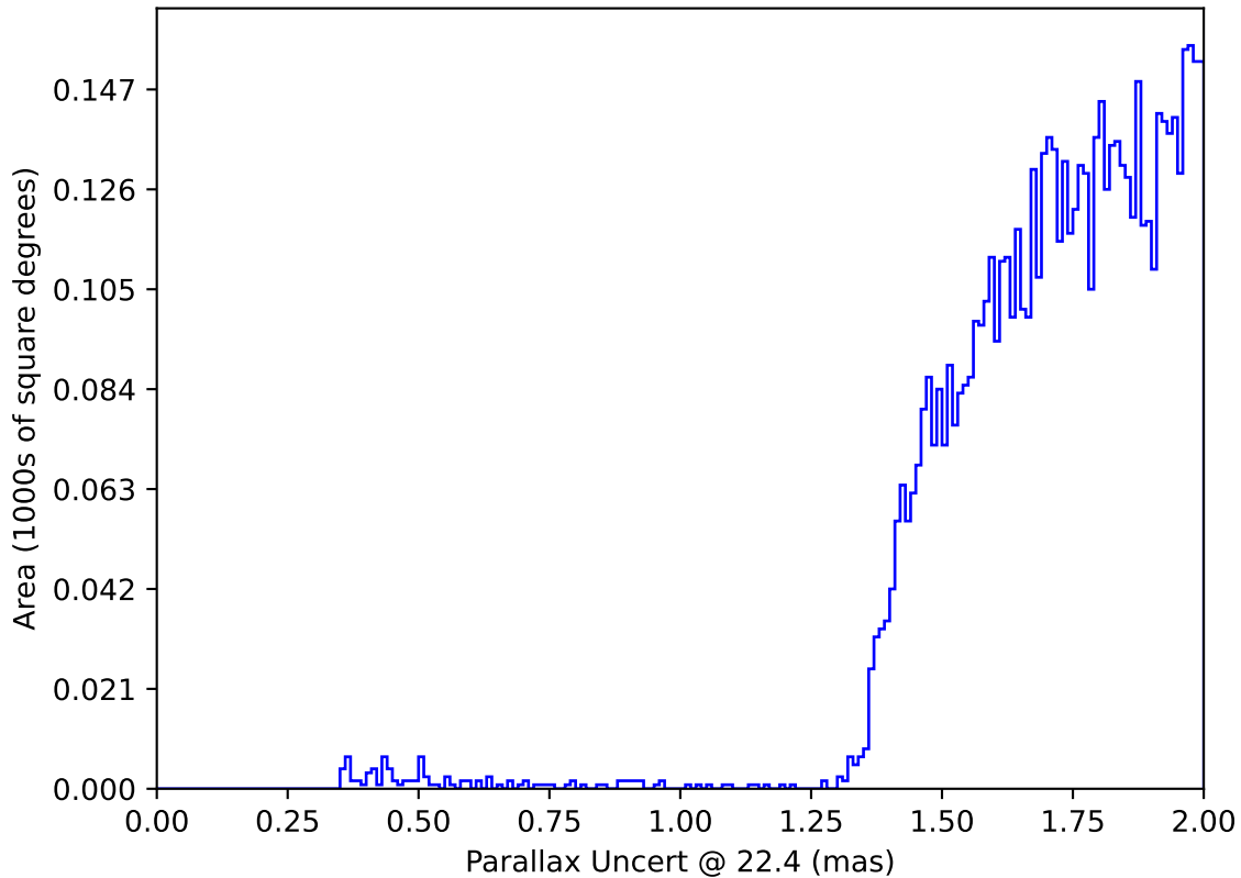
roll_3_v3.4_10yrs : Parallax Uncert @ 22.4
