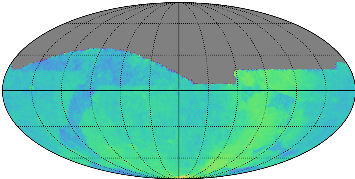
roll_3_v3.4_10yrs : Parallax Coverage @ 22.4
