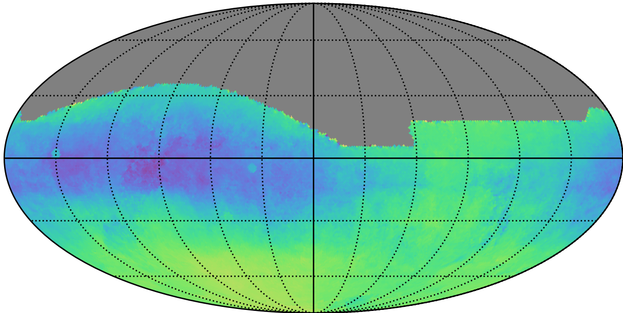
roll_3_v3.4_10yrs : Parallax-DCR degeneracy @ 24.0
