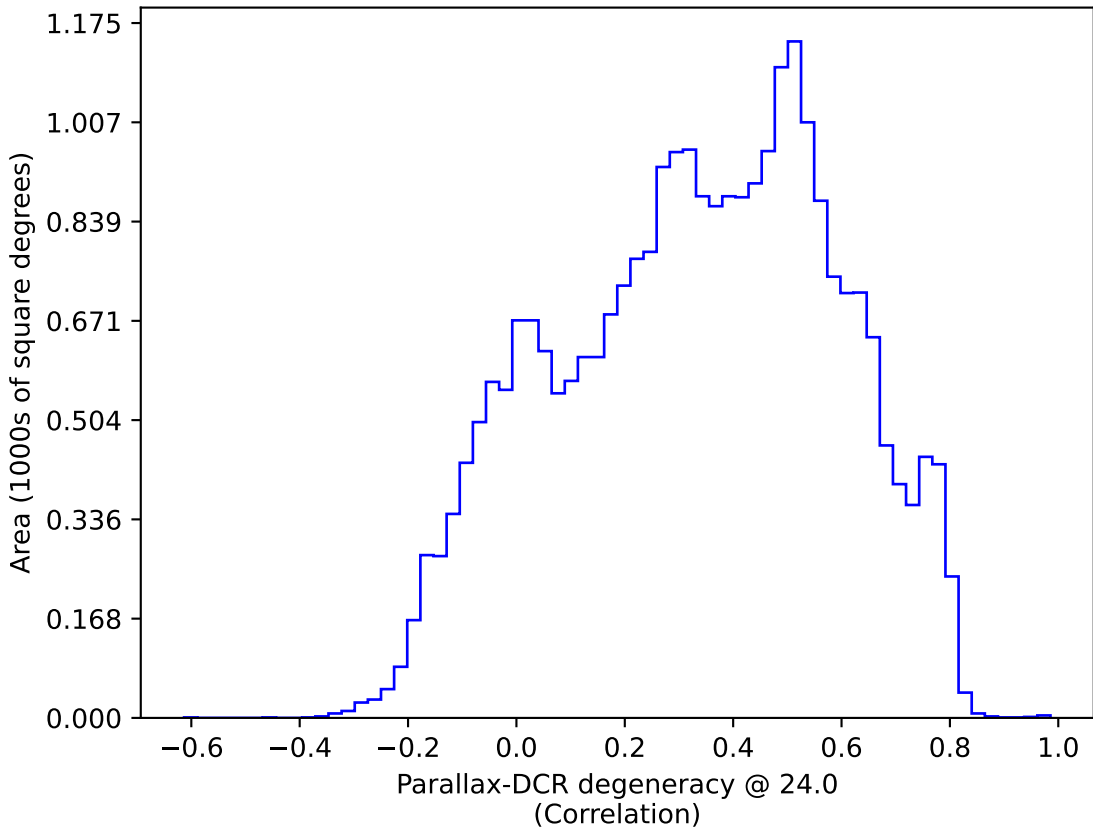
roll_3_v3.4_10yrs : Parallax-DCR degeneracy @ 24.0
