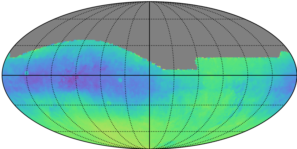
roll_3_v3.4_10yrs : Parallax-DCR degeneracy @ 22.4
