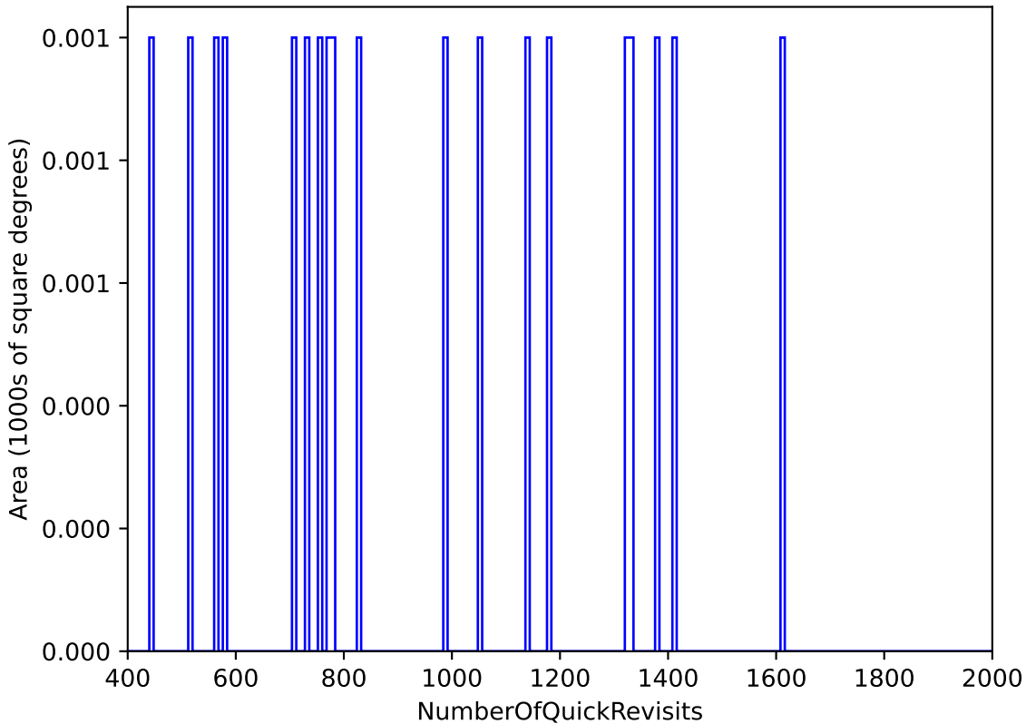
roll_3_v3.4_10yrs : NumberOfQuickRevisits
