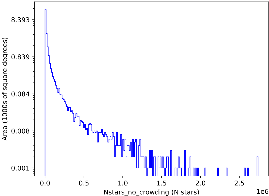
roll_3_v3.4_10yrs u: Nstars_no_crowding
