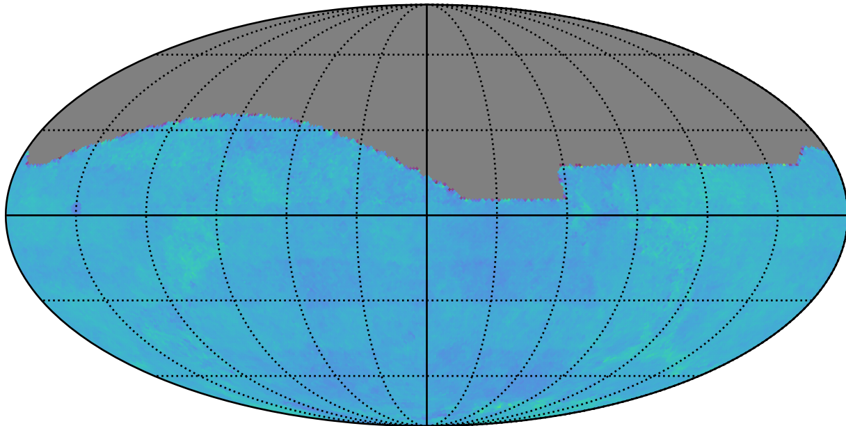
roll_3_v3.4_10yrs : Normalized Proper Motion Uncert @ 24.0
