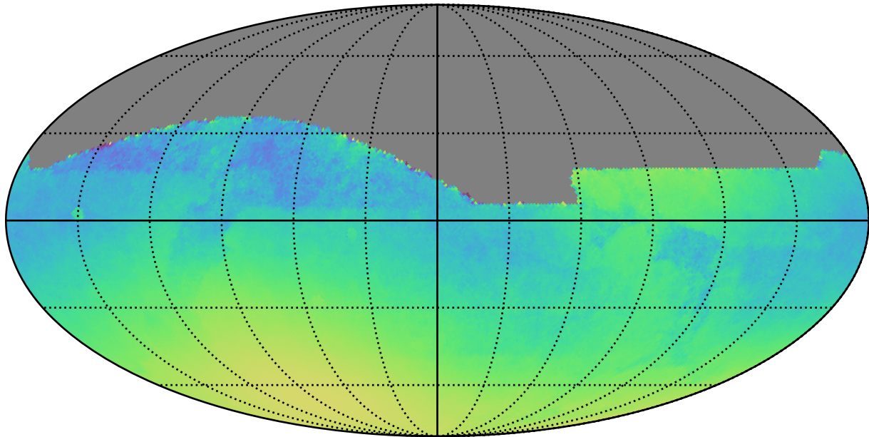
roll_3_v3.4_10yrs : Normalized Parallax Uncert @ 22.4
