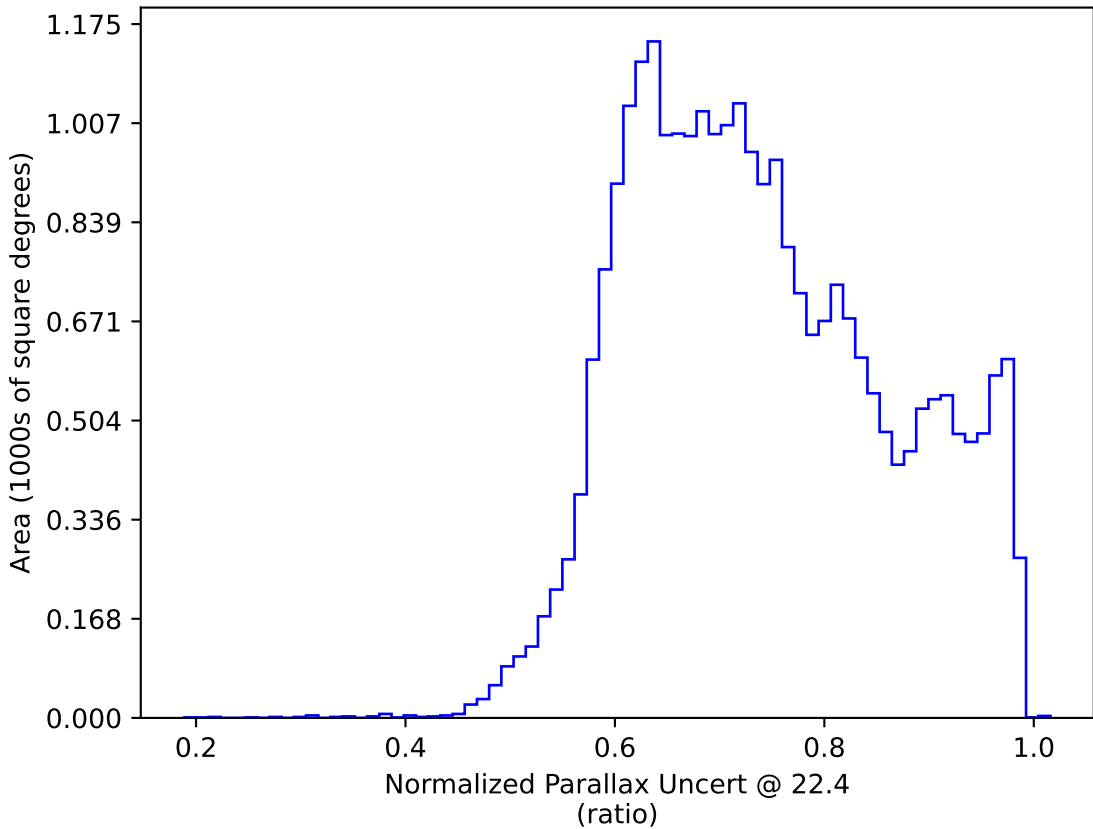
roll_3_v3.4_10yrs : Normalized Parallax Uncert @ 22.4
