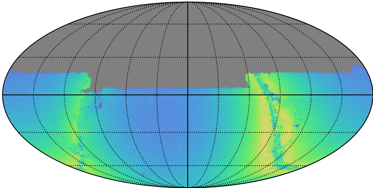
roll_3_v3.4_10yrs u: N stars to Precision 0.20
