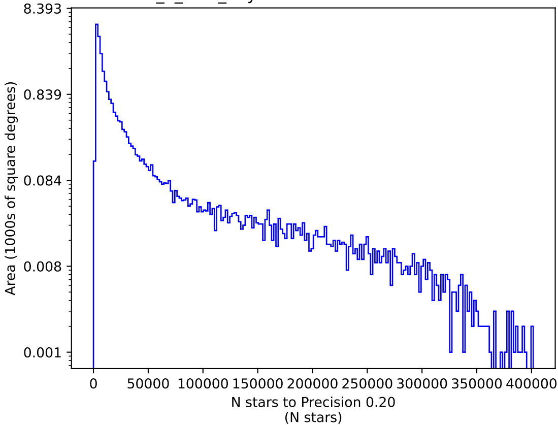
roll_3_v3.4_10yrs u: N stars to Precision 0.20
