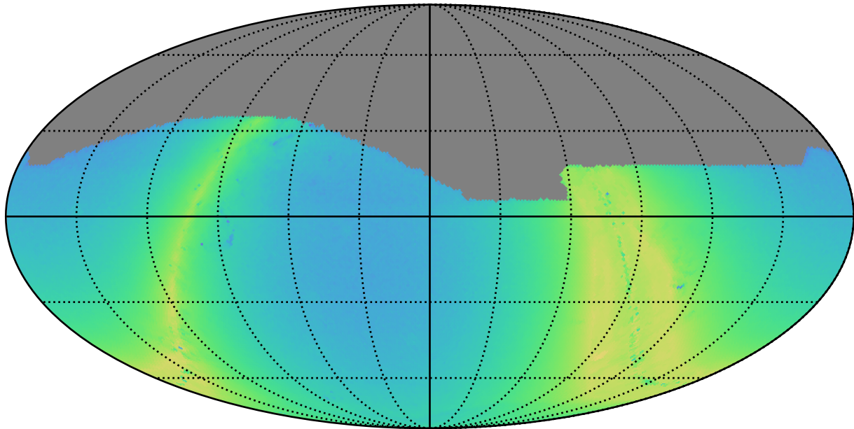
roll_3_v3.4_10yrs r: N stars to Precision 0.20
