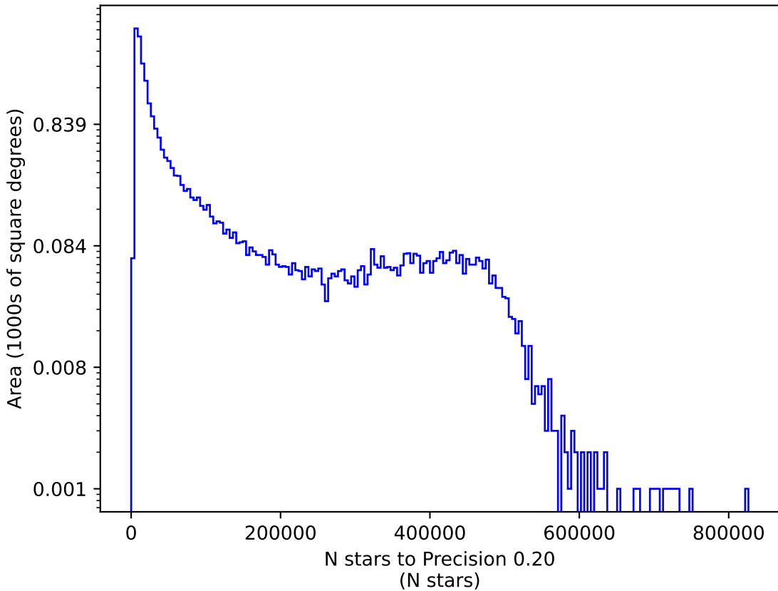
roll_3_v3.4_10yrs r: N stars to Precision 0.20
