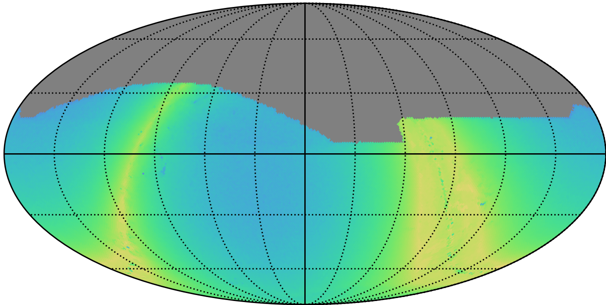
roll_3_v3.4_10yrs i: N stars to Precision 0.20
