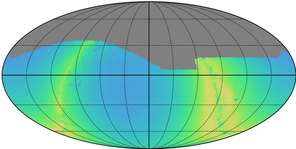
roll_3_v3.4_10yrs g: N stars to Precision 0.20
