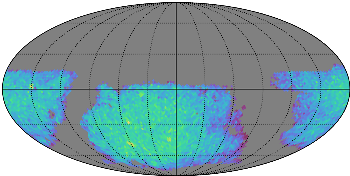
roll_3_v3.4_10yrs gi: LVDwarfs
