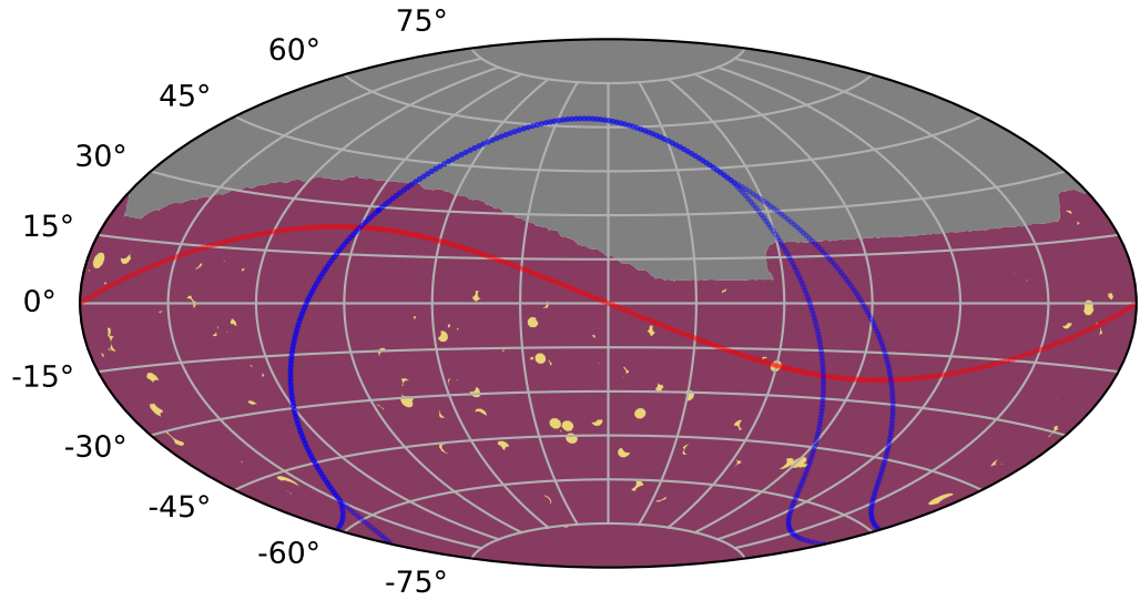
roll_3_v3.4_10yrs all models: KNePopMetric_all_ztfrest_simple_red
