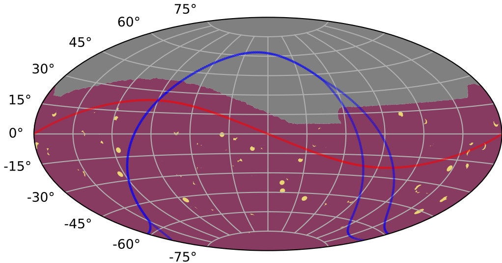
roll_3_v3.4_10yrs all models: KNePopMetric_all_ztfrest_simple_blue
