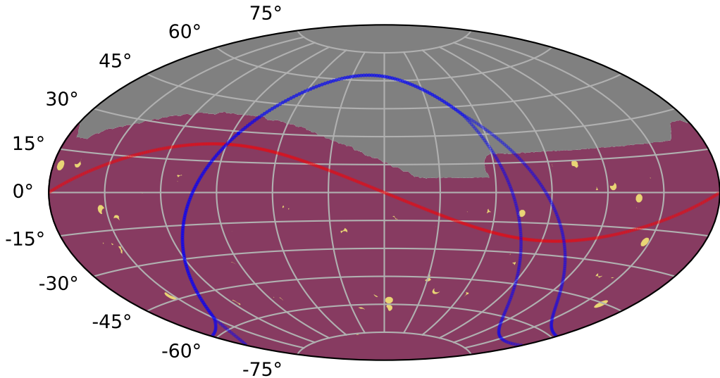
roll_3_v3.4_10yrs all models: KNePopMetric_all_blue_color_detect
