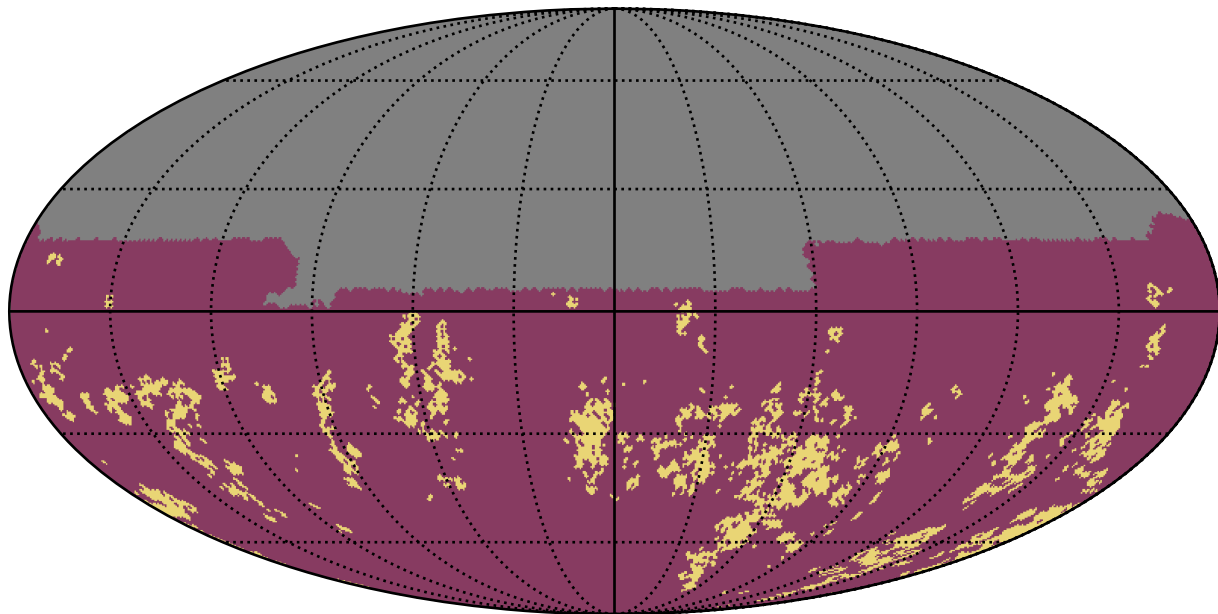
roll_3_v3.4_10yrs u band: Gaps_7hr
