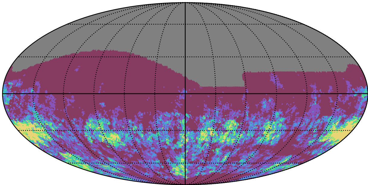
roll_3_v3.4_10yrs r band: Gaps_7hr
