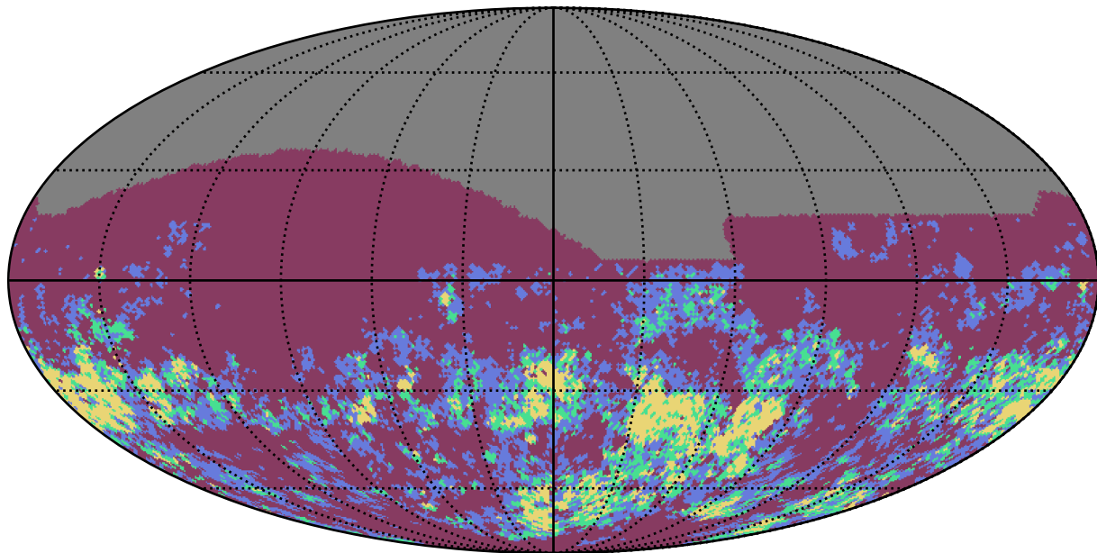
roll_3_v3.4_10yrs i band: Gaps_7hr
