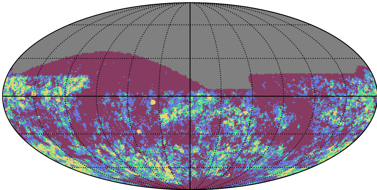
roll_3_v3.4_10yrs z band: Gaps_3hr
