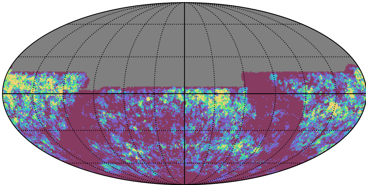
roll_3_v3.4_10yrs y band: Gaps_3hr
