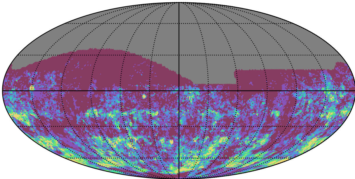
roll_3_v3.4_10yrs r band: Gaps_3hr
