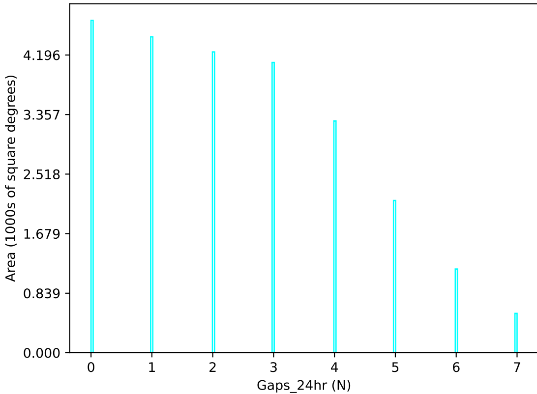
roll_3_v3.4_10yrs u band: Gaps_24hr
