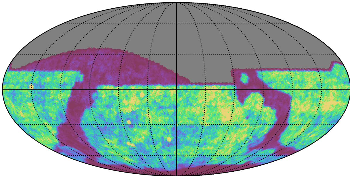
roll_3_v3.4_10yrs r band: Gaps_24hr
