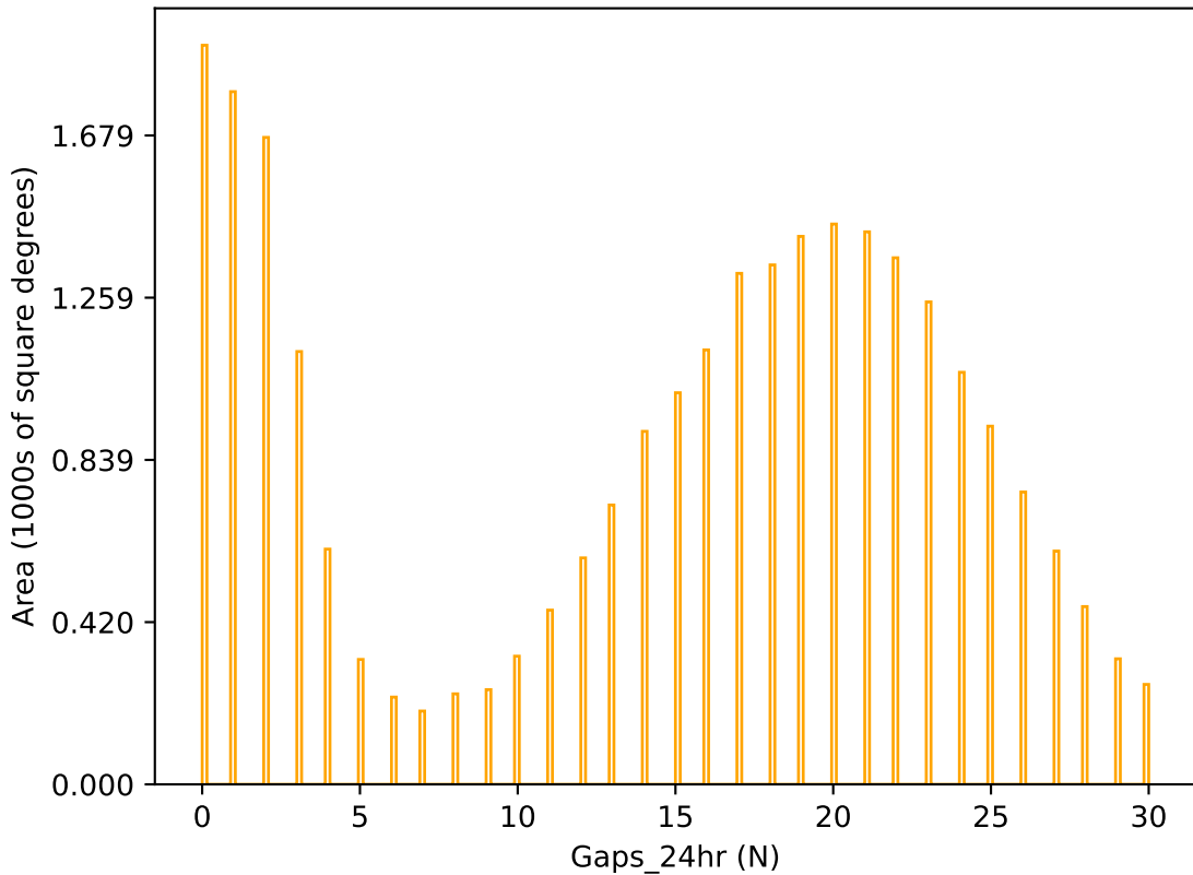
roll_3_v3.4_10yrs r band: Gaps_24hr
