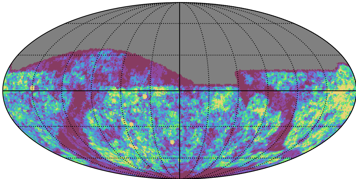
roll_3_v3.4_10yrs g band: Gaps_24hr
