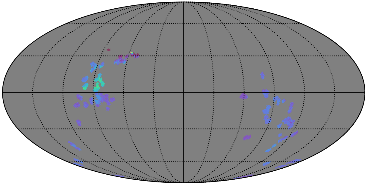
roll_3_v3.4_10yrs : GalplaneTimePerFilter_zucker_sfr_map_g
