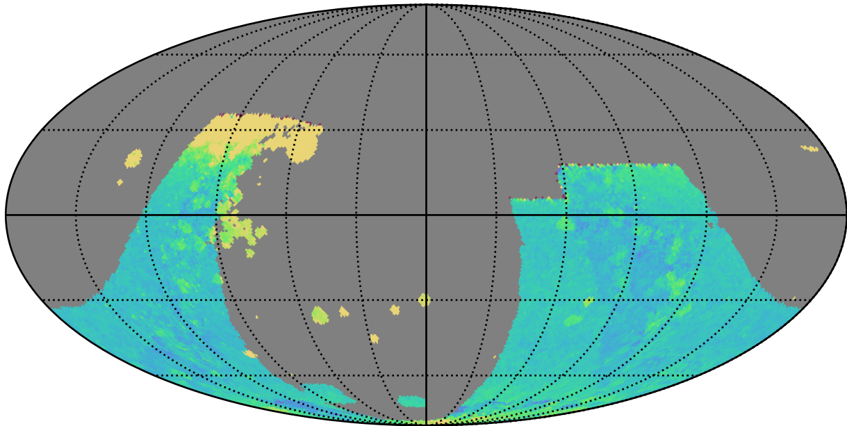
roll_3_v3.4_10yrs : GalplaneTimePerFilter_combined_map_z
