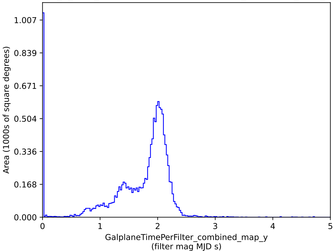
roll_3_v3.4_10yrs : GalplaneTimePerFilter_combined_map_y
