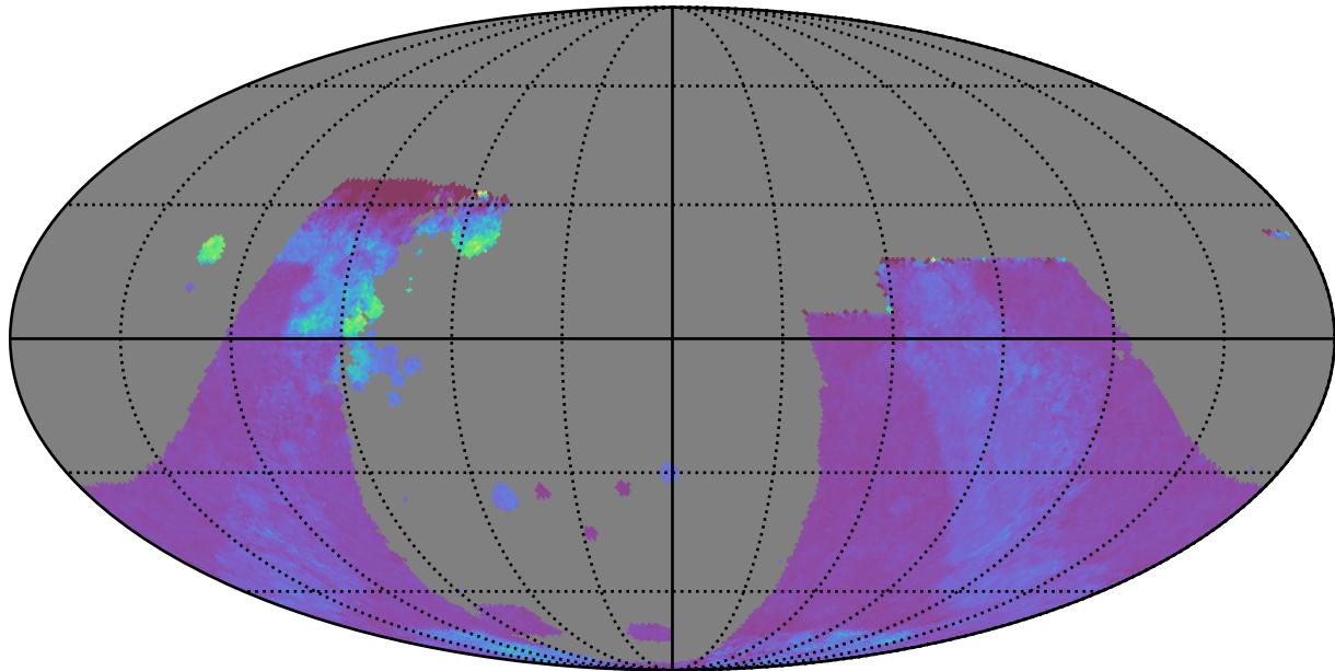
roll_3_v3.4_10yrs : GalplaneTimePerFilter_combined_map_g
