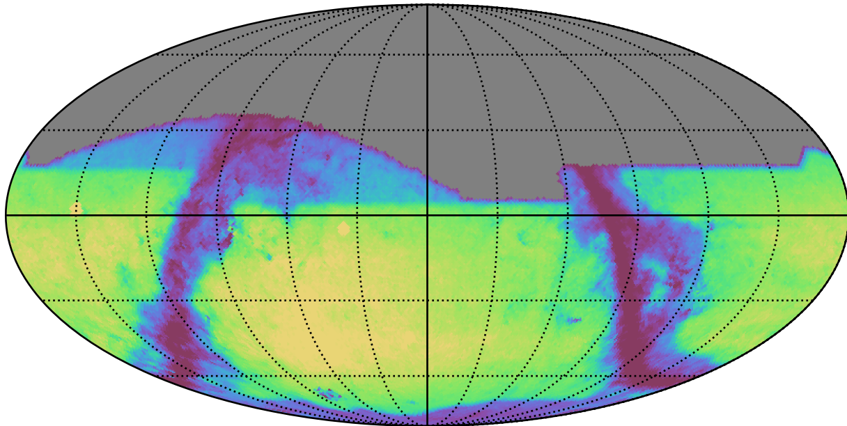
roll_3_v3.4_10yrs r: GalaxyCountsMetricExtended
