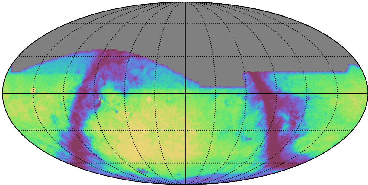
roll_3_v3.4_10yrs g: GalaxyCountsMetricExtended
