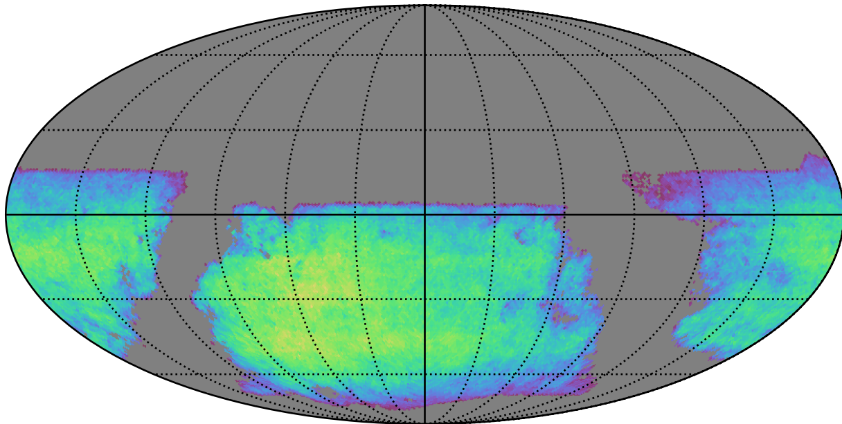
roll_3_v3.4_10yrs i band non-DD year 8: ExgalM5WithCuts
