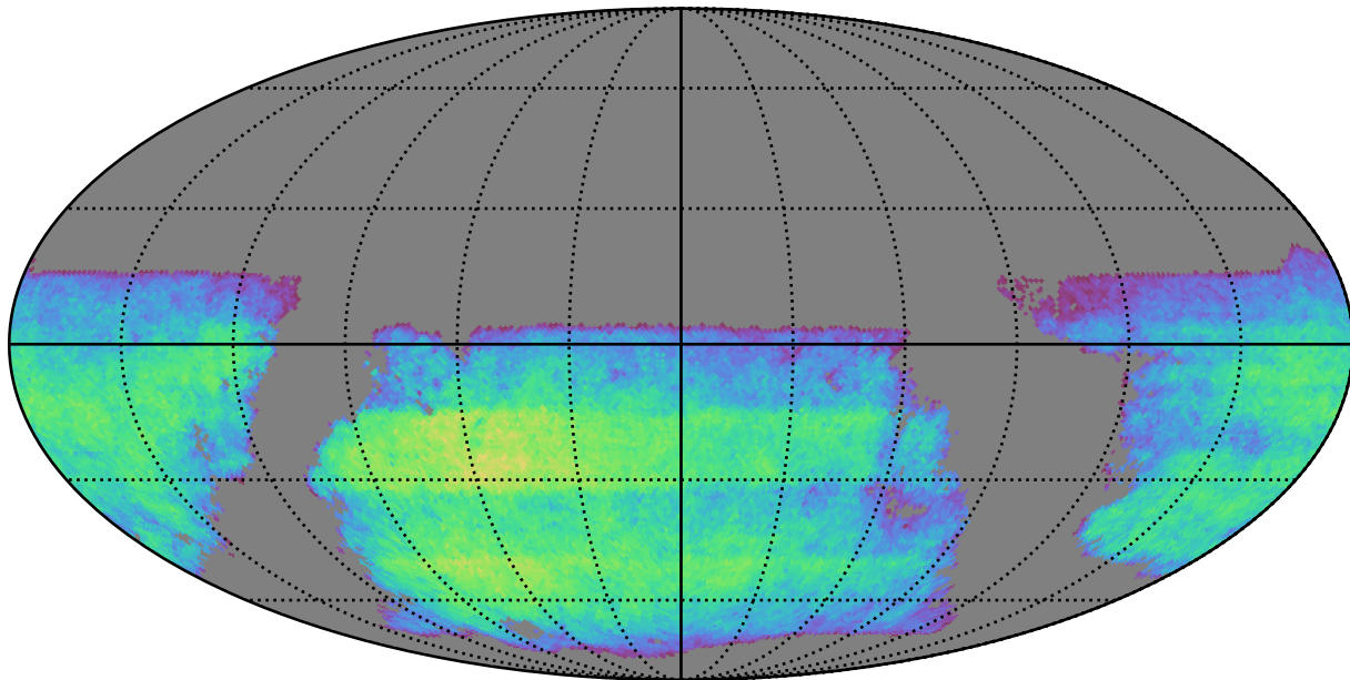
roll_3_v3.4_10yrs i band non-DD year 5: ExgalM5WithCuts
