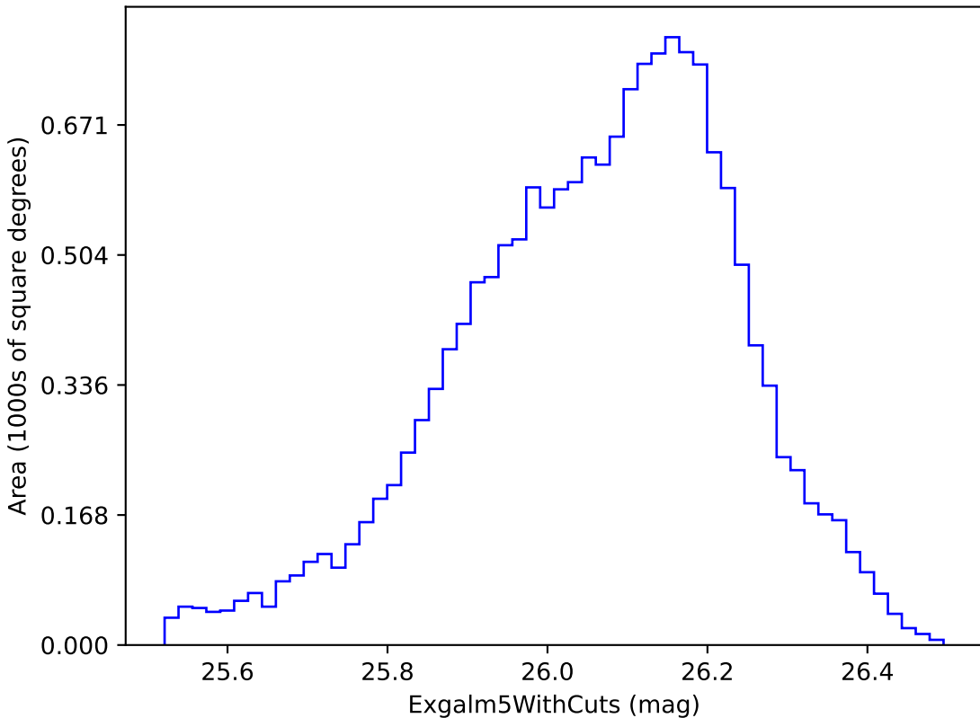
roll_3_v3.4_10yrs i band non-DD year 5: ExgalM5WithCuts
