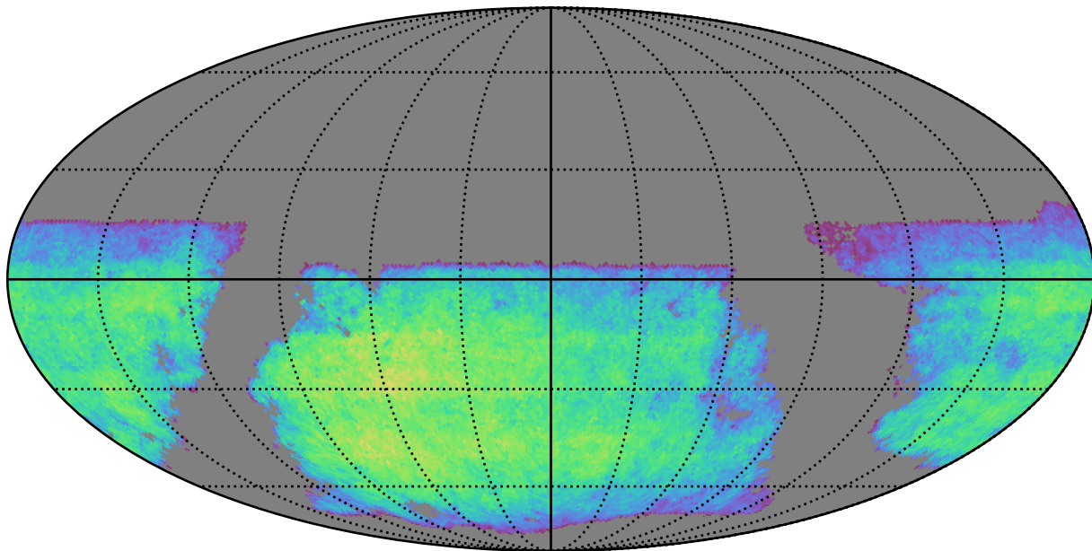
roll_3_v3.4_10yrs i band non-DD year 4: ExgalM5WithCuts
