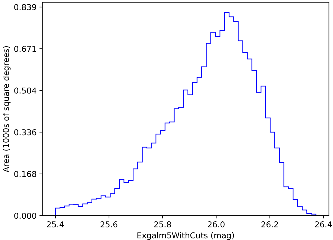
roll_3_v3.4_10yrs i band non-DD year 4: ExgalM5WithCuts
