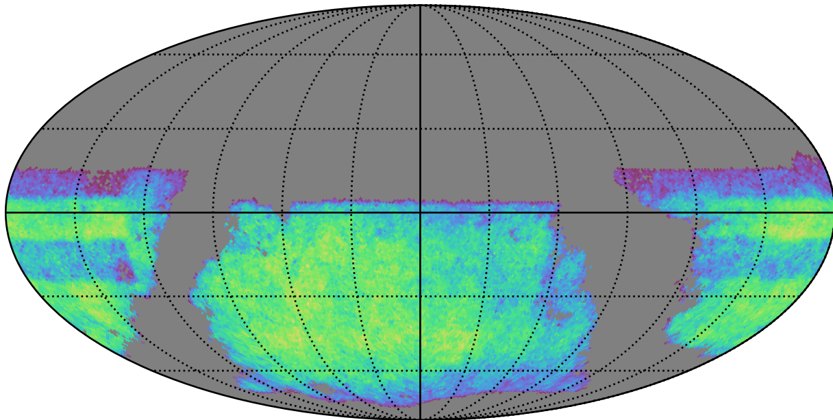
roll_3_v3.4_10yrs i band non-DD year 2: ExgalM5WithCuts
