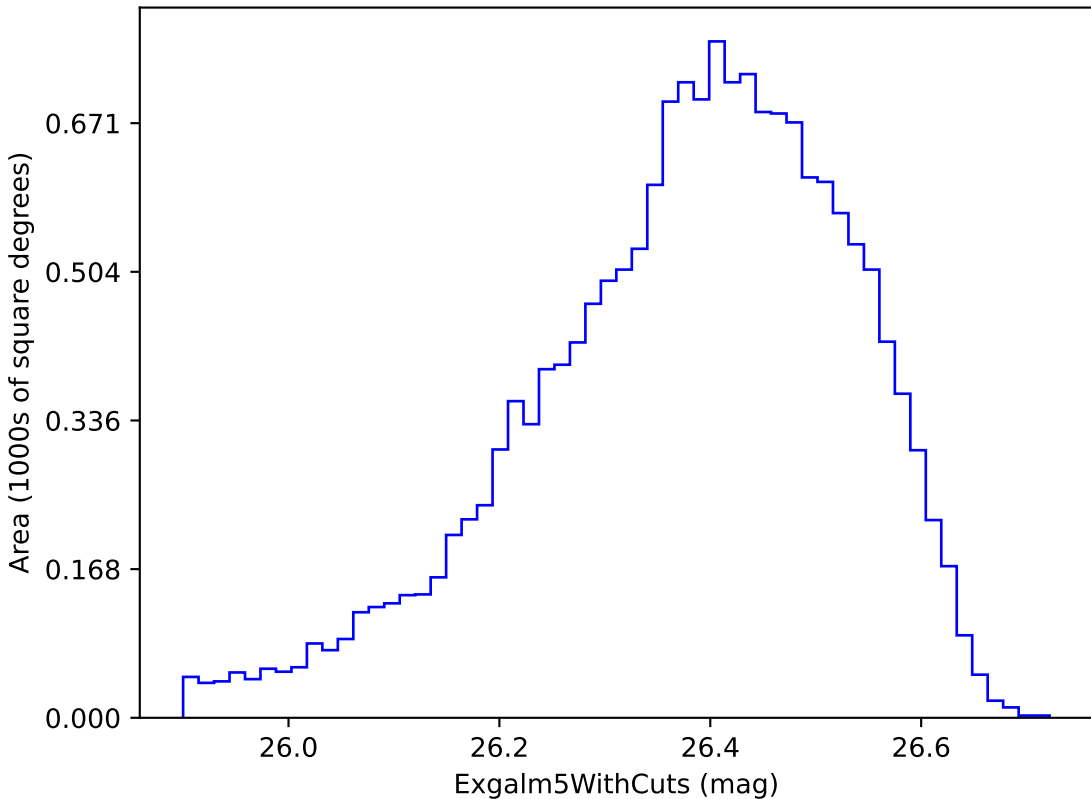
roll_3_v3.4_10yrs i band non-DD year 10: ExgalM5WithCuts
