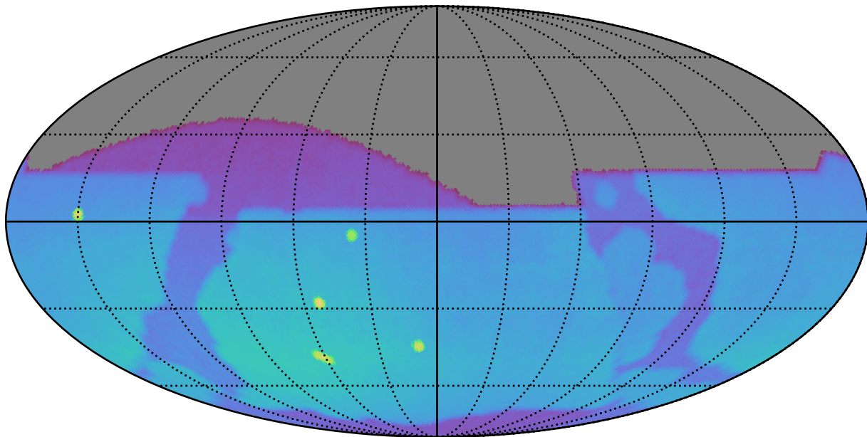
roll_3_v3.4_10yrs : Brown Dwarf, L4
