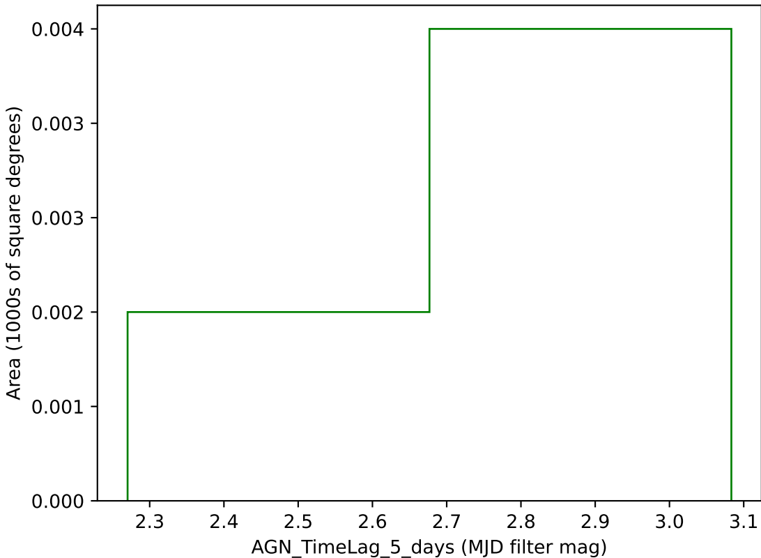
roll_3_v3.4_10yrs g band: AGN_TimeLag_5_days
