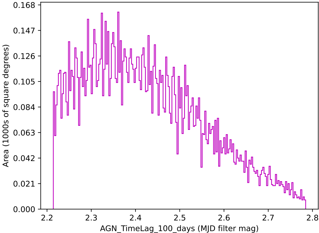
roll_3_v3.4_10yrs z band: AGN_TimeLag_100_days
