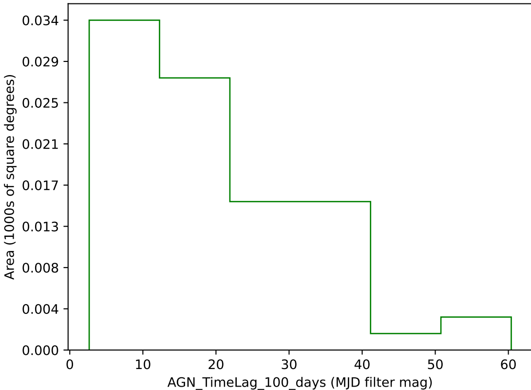
roll_3_v3.4_10yrs g band: AGN_TimeLag_100_days
