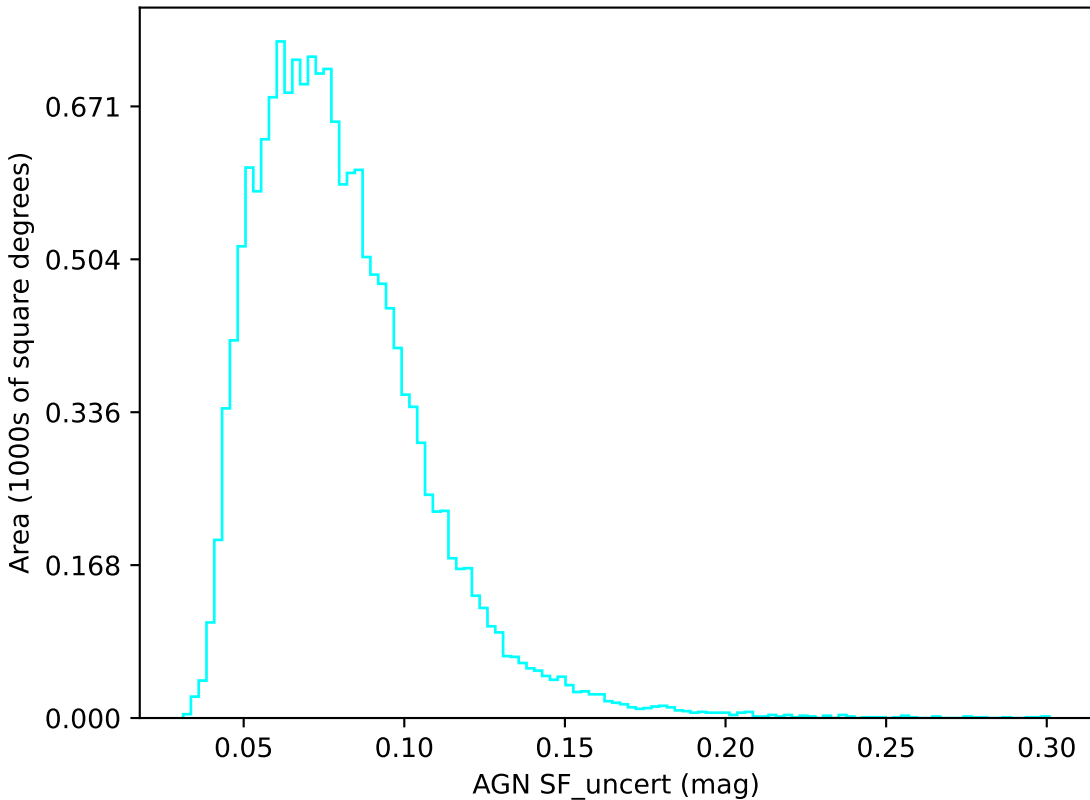
roll_3_v3.4_10yrs u band: AGN SF_uncert
