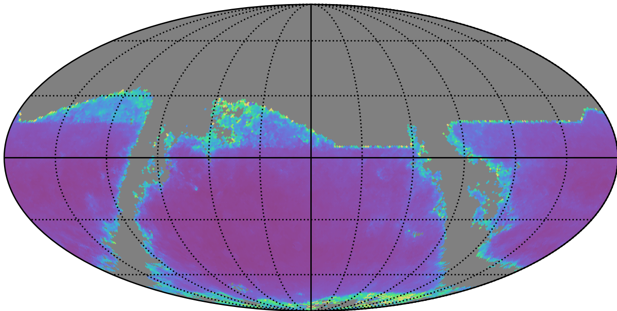
roll_3_v3.4_10yrs r band: AGN SF_uncert
